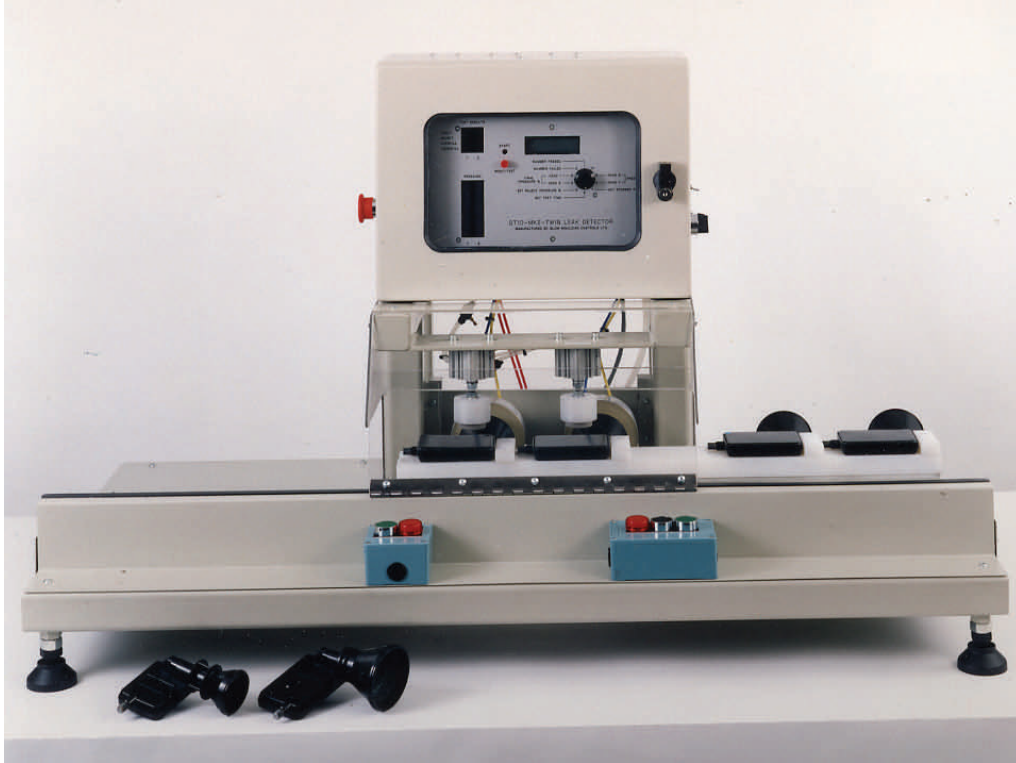
Shuttle table hand loaded leak tester. Shown here testing microwave 'LNB' modules
